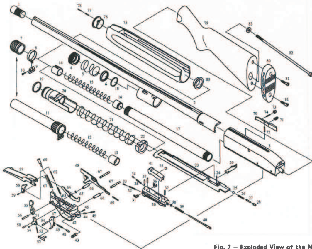
Fig. 2 - Exploded View of the MP-153
